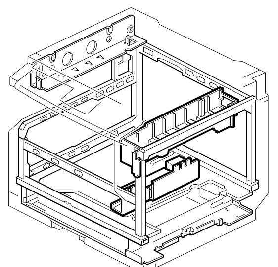
18.FRAME SECTION (B001)
