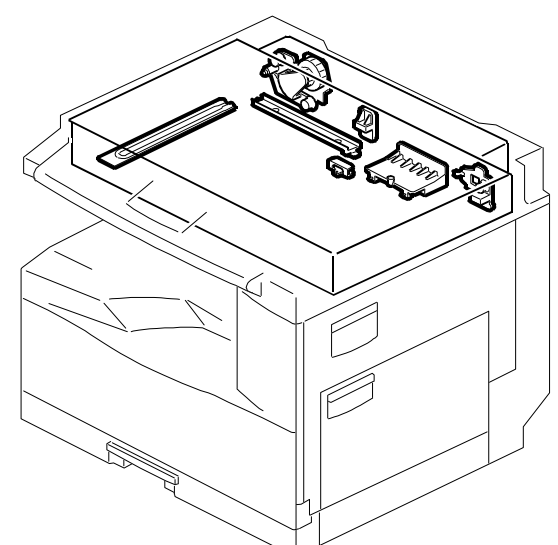
6.SCANNER SECTION 3 (B001)
