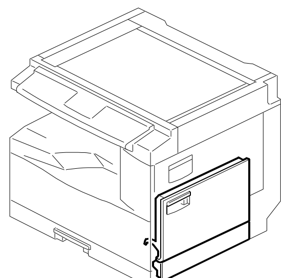
12.BY-PASS FEED SECTION (B001)
