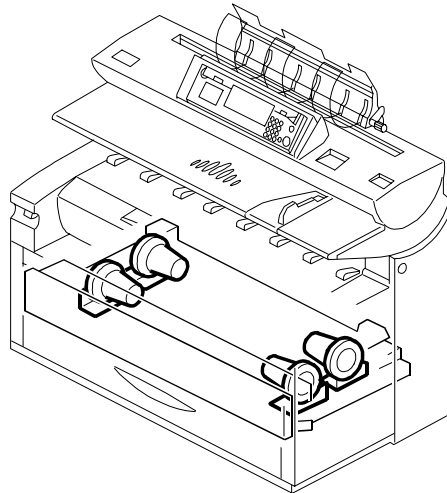
16. PAPER TRAY UNIT 6 (B010)
