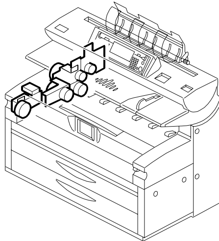
28. DRIVE SECTION (B010)
