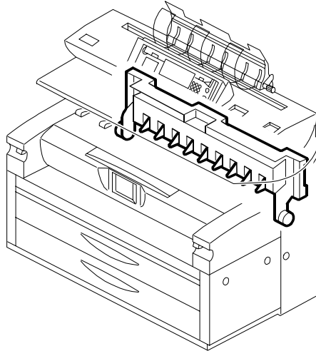
26. PAPER EXIT SECTION 1 (B010)
