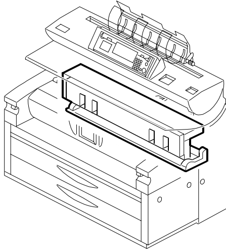
25. FUSING UNIT 3 (B010)
