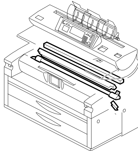
10. CHARGE CORONA SECTION (B010)
