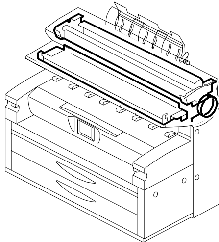
4. OPTICAL SECTION 1 (B010)
