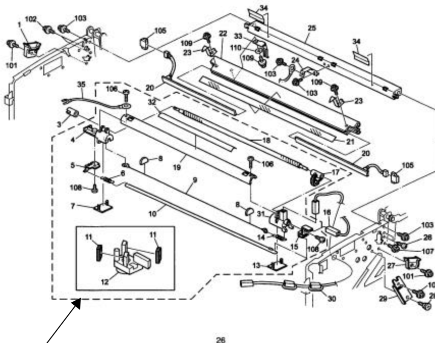
10.CHARGE CORONA SECTION (B010)
