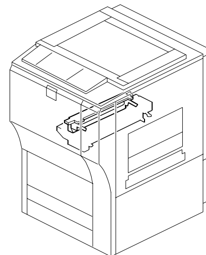
48. Fusing Unit 2 (B132/B181/B200)
