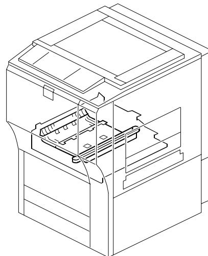
59. Duplex Unit 5 (B132/B181/B200)
