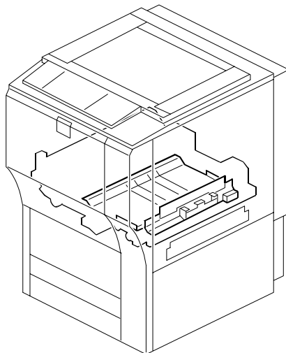
44. Transfer Entrance 3 (B132/B181/B200)
