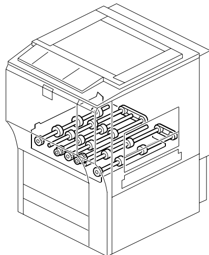
58. Duplex Unit 4 (B132/B181/B200)
