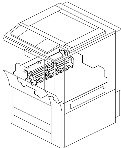
52. Paper Exit 2 (B132/B181/B200)
