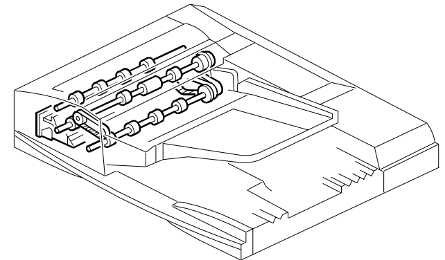
9. Original Trans 2 (B132/B181/B200)
