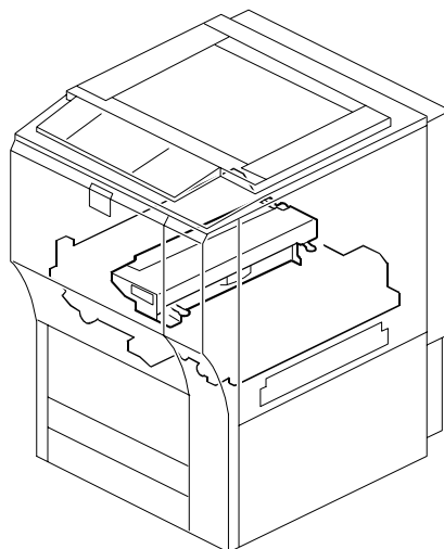
47. Fusing Unit 1 (B132/B181/B200)
