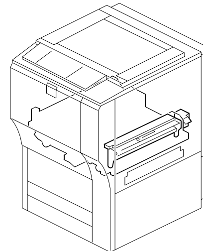
42. Transfer Entrance 1 (B132/B181/B200)
