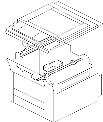
54. Paper Exit 4 (B132/B181/B200)
