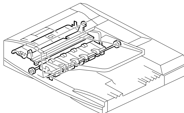
11. Original Exit 1 (B132/B181/B200)
