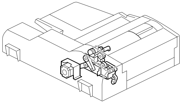
13. ARDF Drive & Electrical 1
