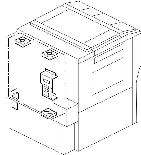
69. Electrical Section 3 (B132/B181/B200)
