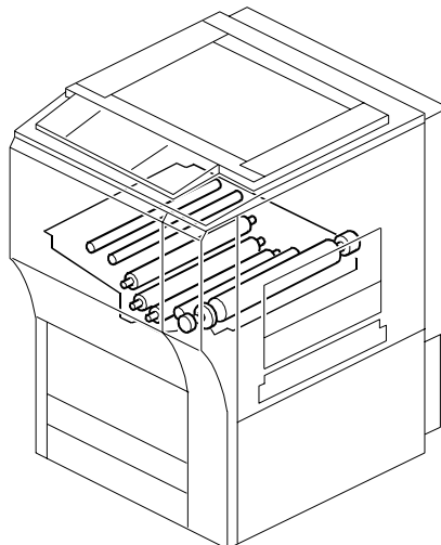
38. Transfer Belt Unit 2 (B132/B181/B200)
