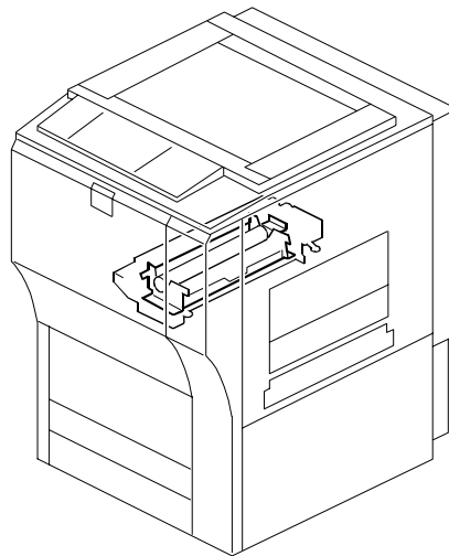
50. Fusing Unit 4 (B132/B181/B200)
