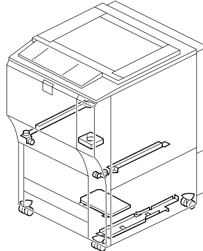
77. Frame Section 3 (B132/B181/B200)
