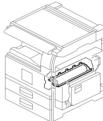
18. OPC UNIT 2 (B291/B295/B296/B297)
