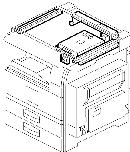
5. OPTICS UNIT 1 (B195/B198/B264/B265)
