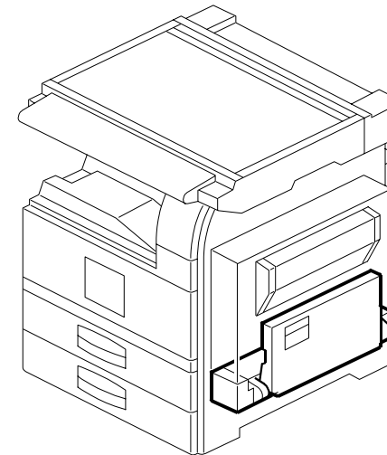
9. BY-PASS FEED UNIT 1 (B195/B198/B264/B265)
