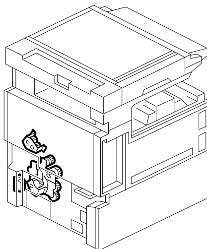
29. DRIVE SECTION 3 (B195/B198/B264/B265)
