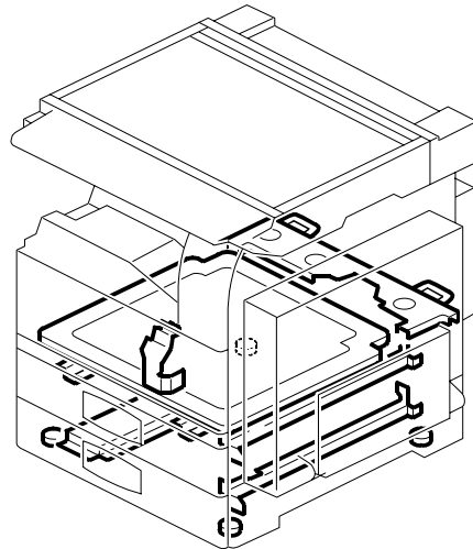
34. FRAME SECTION 2 (B195/B198/B264/B265)
