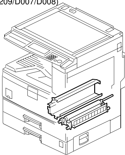
14. PAPER REGISTRATION (B205/B209/D007/D008)
