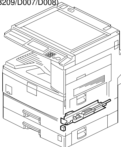
11. PAPER FEED SECTION 2 (B205/B209/D007/D008)
