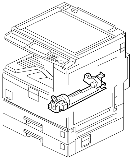
13. TONER HOPPER UNIT (B205/B209/D007/D008)
