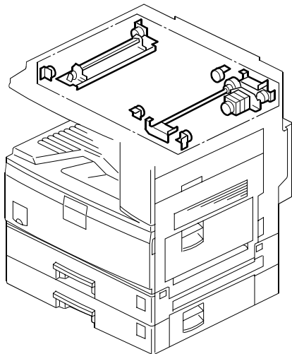
7. OPTICS SECTION 3 (B205/B209/D007/D008)
