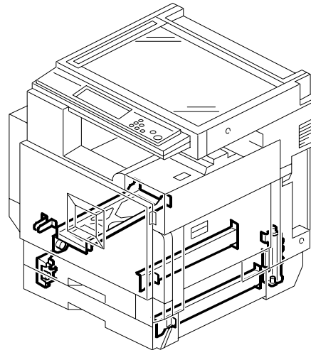
47. Frame Section 3
