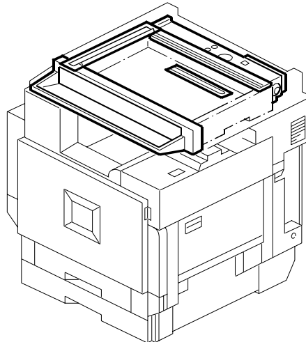
5. Scanner Section 1
