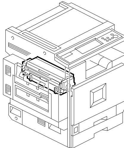
26. Fusing Unit 1 (B146/B147/B148/B149)
