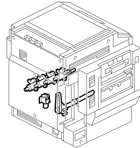
39. Drive Section 2 (B146/B147/B148/B149)
