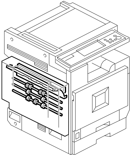
34. Duplex unit 2 (B146/B147/B148/B149)
