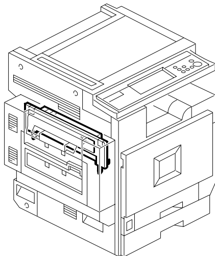
28. Paper Exit Section 1
