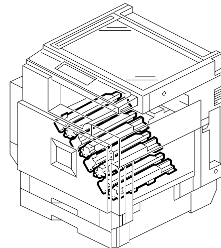
21. PCU/Development Unit
