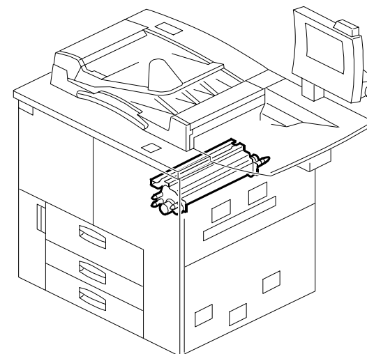
36. DEVELOPMENT UNIT 1 (B070/B071)
