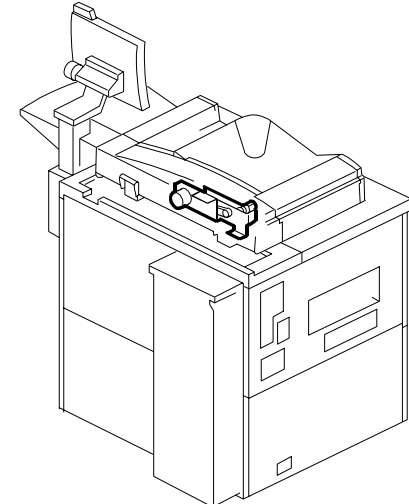
12. DF DRIVE SECTION 1 (B070/B071)
