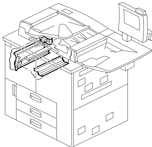
50. PAPER EXIT SECTION 2 (B070/B071)
