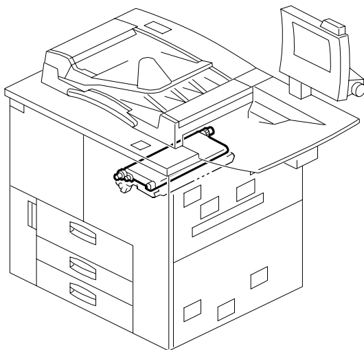
43. TRANSFER BELT UNIT 1 (B070/B071)
