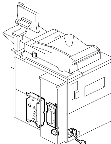
65. ELECTRICAL SECTION 3 (B070/B071)
