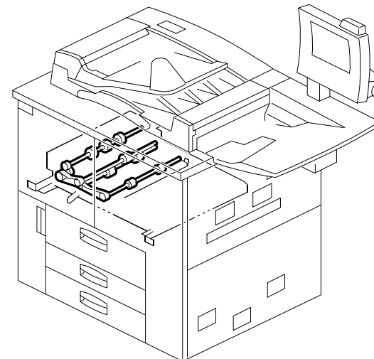
57. DUPLEX UNIT 5 (B070/B071)
