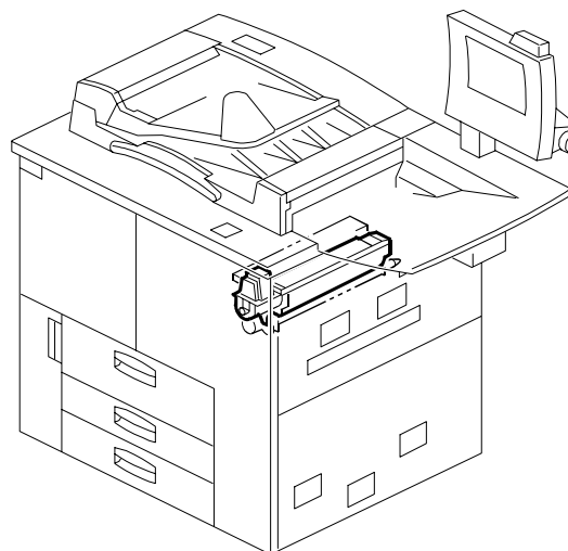
35. TONER HOPPER SECTION
