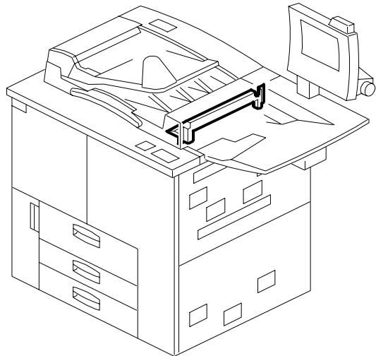
10. ORIGINAL EXIT 1 (B070/B071)
