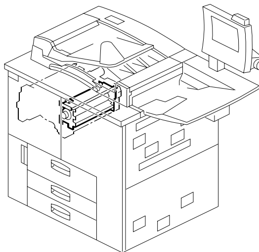
47. FUSING UNIT 3 (B070/B071)
