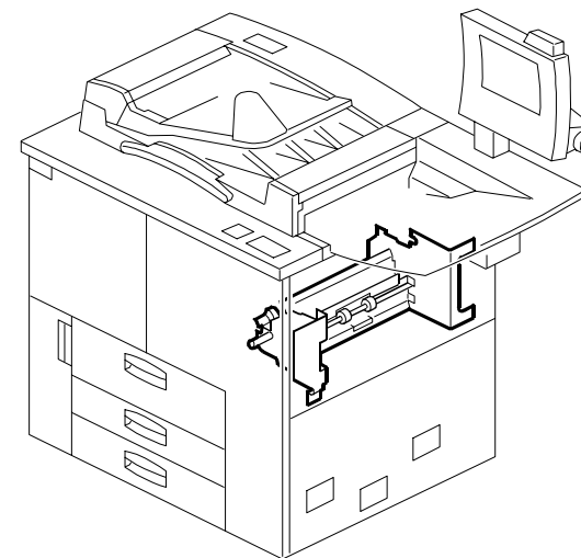
30. PAPER REGISTRATION 3 (B070/B071)
