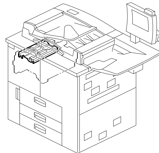
51. PAPER EXIT SECTION 3 (B070/B071)
