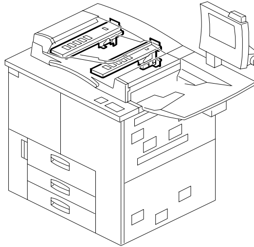
14. DF FRAME SECTION (B070/B071)
