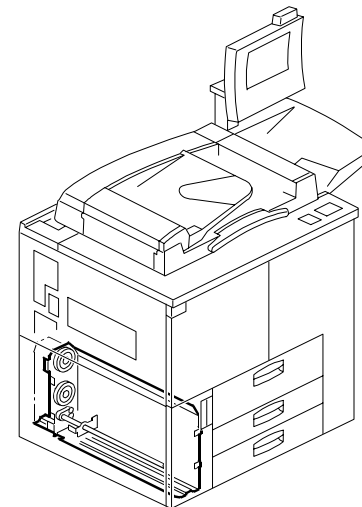
33. TONER SUPPLY UNIT 1 (B070/B071)
