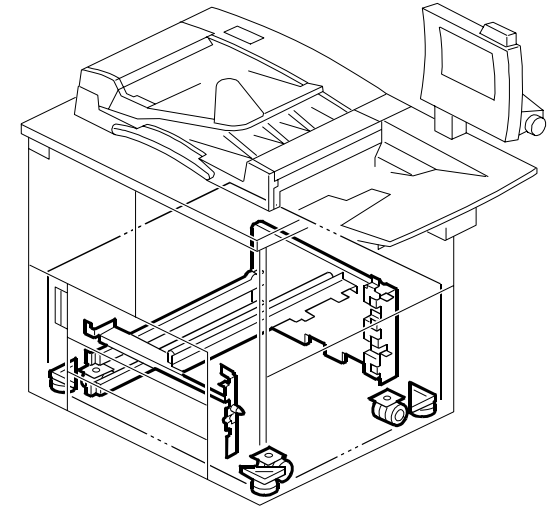
75. FRAME SECTION 5 (B070/B071)
