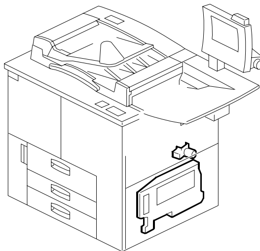
38. TONER COLLECTION BOTTLE
