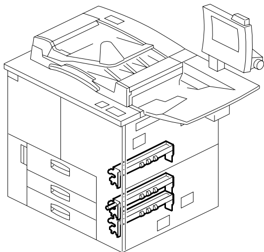
25. PAPER FEED UNIT 2 (B070/B071)
