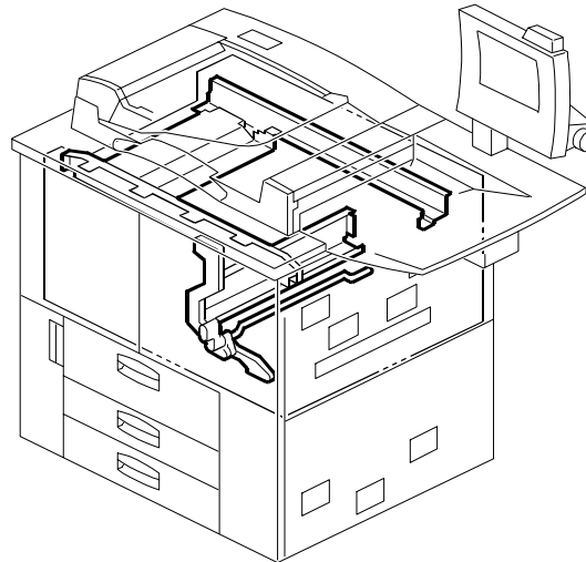
71. FRAME SECTION 1 (B070/B071)
