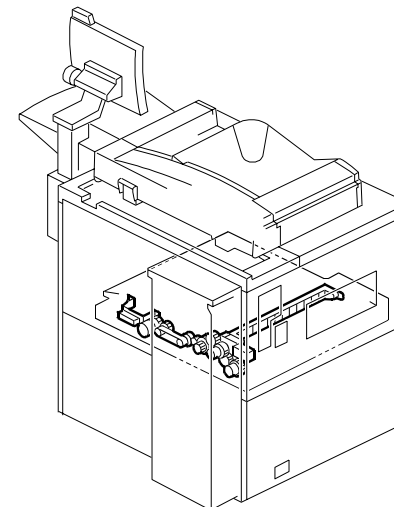
54. DUPLEX UNIT 2 (B070/B071)
