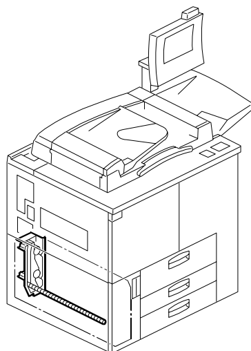
34. TONER SUPPLY UNIT 2 (B070/B071)
