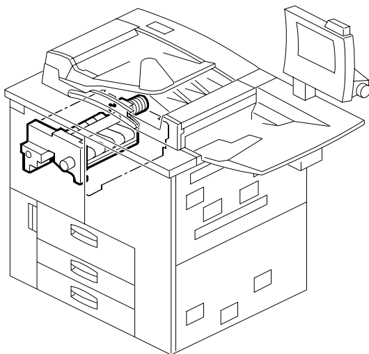
49. PAPER EXIT SECTION 1 (B070/B071)
