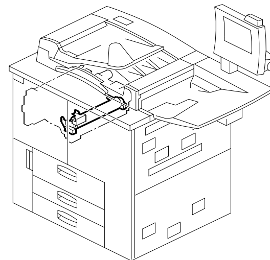
48. FUSING UNIT 4 (B070/B071)
