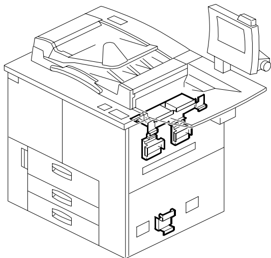
67. ELECTRICAL SECTION 5 (B070/B071)
