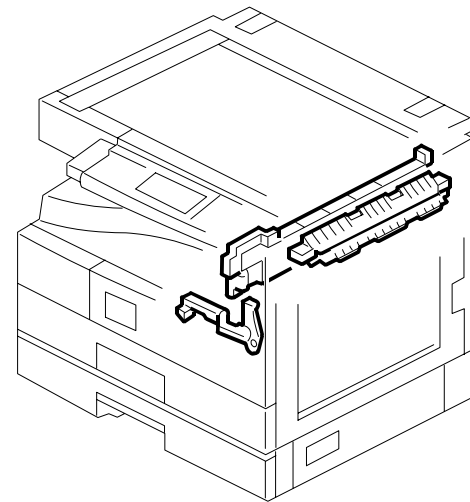
18. PAPER EXIT SECTION (B26064/B26164)
