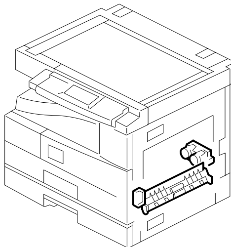
11. 1ST PAPER FEED SECTION (B26064/B26164)
