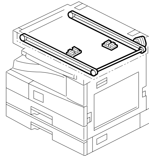
6. OPTICS SECTION 3 (B26064/B26164)
