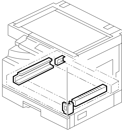
26. FRAME SECTION 2 (B122/B123/B260/B261)
