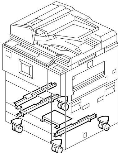
70. LOWER FRAME 2
