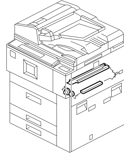
33. DEVELOPMENT UNIT 1
