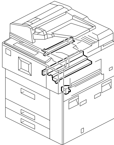
67. UPPER FRAME 2
