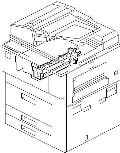
46. FUSING UNIT 4 (Model C2)
