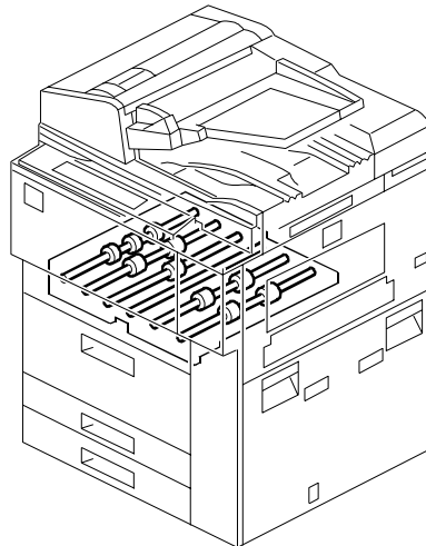
53. DUPLEX UNIT 4
