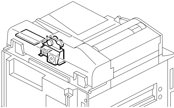
13. DF DRIVE/ELECTRICAL 2
