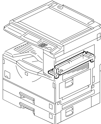
17. FUSING UNIT 2 (B089/B093/B097)
