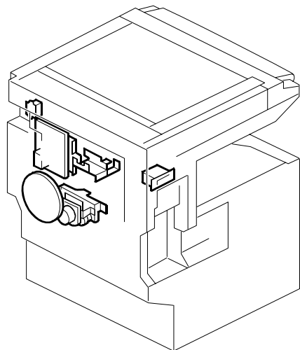
22. DRIVE SECTION 4 (B089/B093/B097)
