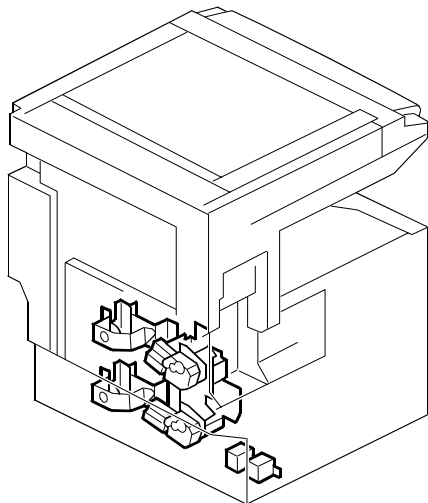
19. DRIVE SECTION 1 (B089/B093/B097)
