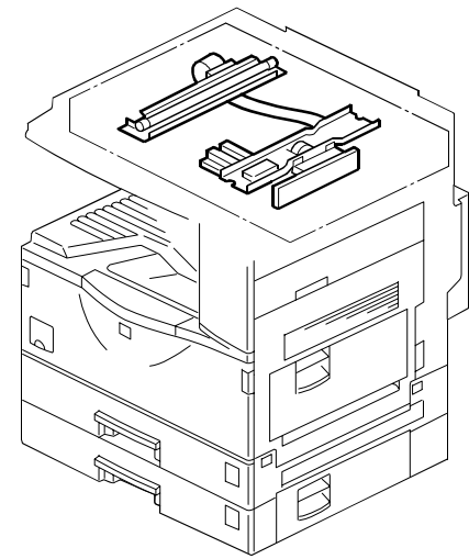
6. OPTICS SECTION 2 (B022/B027)
