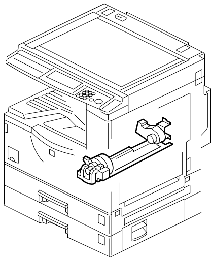
13. TONER HOPPER UNIT (B022/B027)
