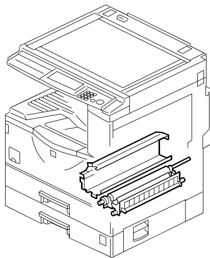
14. PAPER REGISTRATION (B022/B027)
