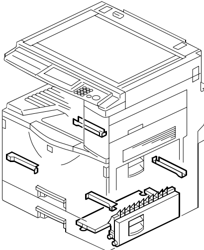
10. PAPER FEED SECTION 1 (B022/B027)
