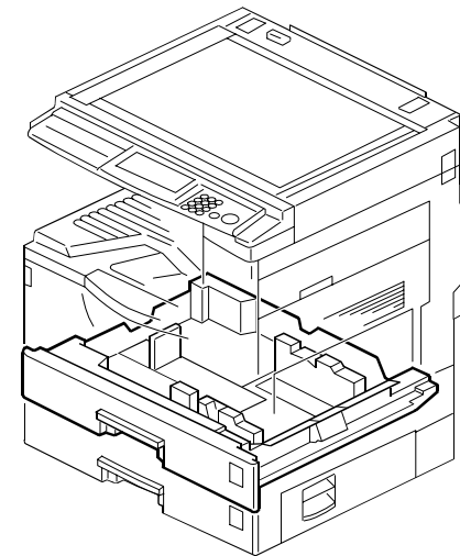
15. PAPER TRAY (B022/B027)
