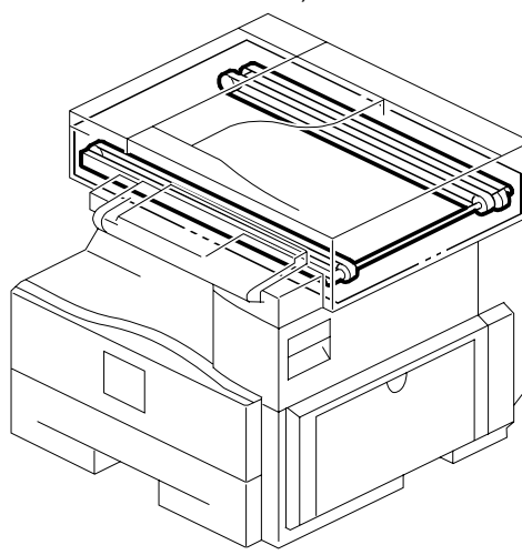
12. OPTICS SECTION 2 (B129/B130/B168/B169)
