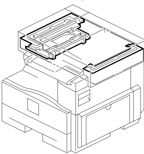
11. OPTICS SECTION 1 (B129/B130/B168/B169)
