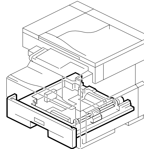
6. PAPER CASSETTE (B129/B130/B168/B169)
