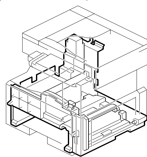
18. FRAME SECTION (B129/B130/B168/B169)
